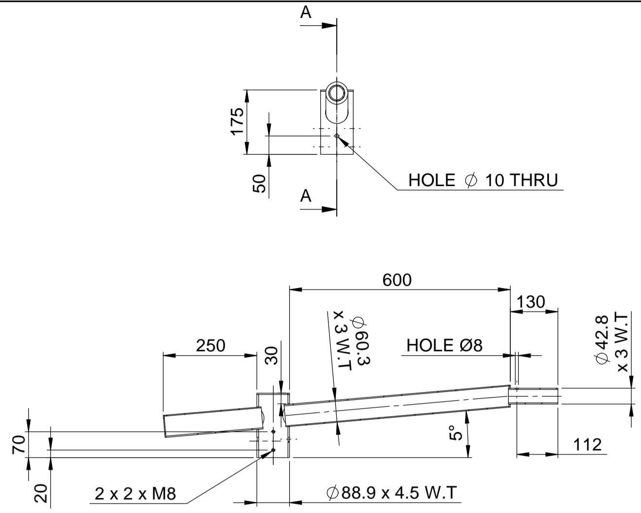
ARM SCALE 1:10
